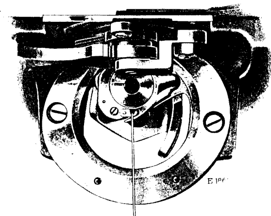
FIG. 9. SHUTTLE THREADED
